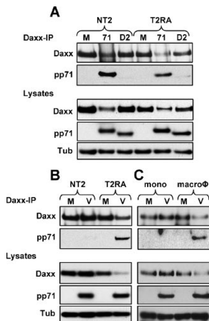
FIG. 3. Tegument-delivered pp71 fails to bind Daxx in undifferentiated NT2 and THP-1 cells. (A) NT2 cells were mock transduced (lane M) or transduced with an rAD expressing either pp71 (lane 71) or the pp71 Daxx-binding mutant (lane D2) at 2,000 or 6,000 particles per cell (ppc), respectively, for 24 h, while differentiated T2RA cells were transduced with pp71 (lane 71) or the pp71 Daxx-binding mutant (lane D2) at 500 or 1,000 ppc, respectively, for 12 h. Lysates were harvested and used in a co-IP/Western blot assay. Lysates were immunoprecipitated with an antibody to Daxx. (B) NT2 or differentiated T2RA cells were mock infected (lane M) or infected with HCMV (lane V) at an MOI of 3 or 1, respectively. Lysates were harvested at 6 hpi and used in a co-IP/Western blot assay. Lysates were immunoprecipitated with an antibody to Daxx. (C) THP-1 monocytes (mono) or THP-1-derived macrophages (macro \Phi ) were mock infected (lane M) or infected with HCMV (lane V) at an MOI of 3 for 12 h. Lysates were harvested and used in a co-IP/Western blot assay. Lysates were immunoprecipitated with an antibody to Daxx. Result from one experiment is shown. Tub, tubulin.
