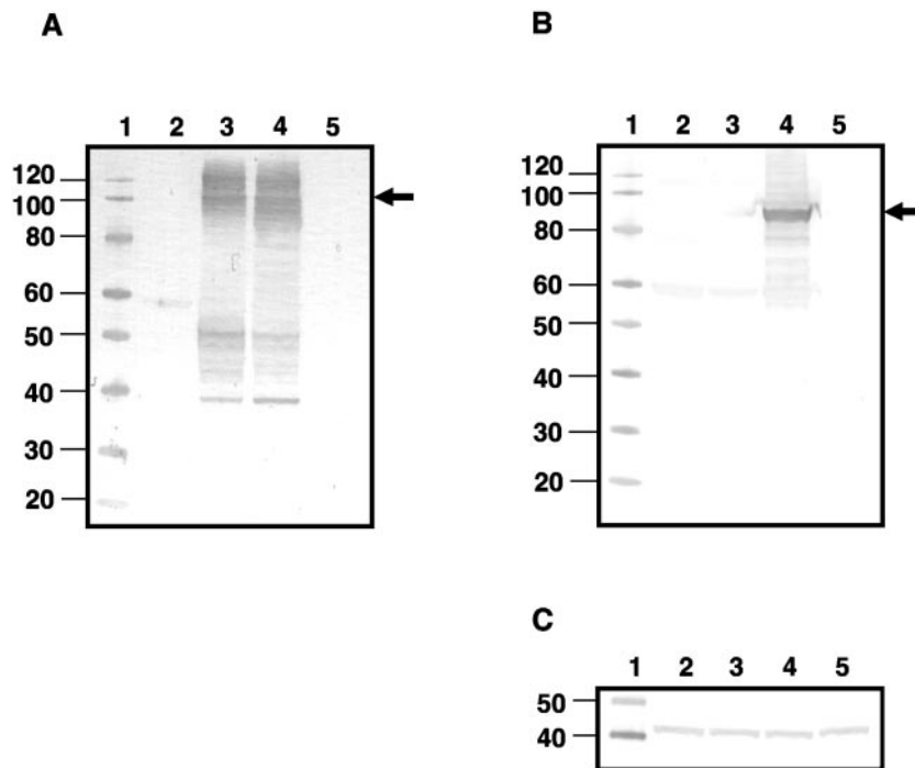
FIG. 3. Western blot analysis of cell-associated EV GP and NP expressed by the recombinant vectors. LLC-MK2 cells were infected with the recombinant viruses, and total cell lysates were prepared 24 h later, separated by electrophoresis on 4 to 12% bis-Tris acrylamide gradient gels under denaturing and reducing conditions, and subjected to Western blot analysis. Replicate blots were analyzed with rabbit anti-EV antibodies (A), guinea pig anti-NP antibodies (B), and a mouse monoclonal antibody against actin as a loading control (C). Lanes: 1, molecular weight markers; 2, HPIV3; 3, HPIV3/EboGP; 4, HPIV3/EboGP-NP; 5, mock infection. Molecular masses of the marker proteins (in kilodaltons) are shown in the left margins, and the positions of EV GP1 (A) and NP (B) are indicated with arrows.
