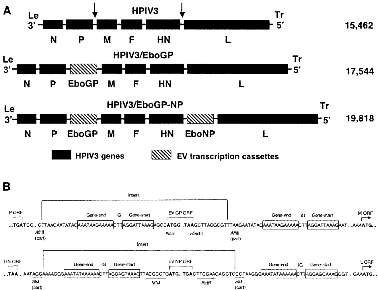
FIG. 1. Genome structures of recombinant HPIV3s expressing EV GP and NP. (A) Schematic diagrams of the genome of the HPIV3 vector, with insertion sites indicated by arrows (top) and HPIV3 vectors containing a transcription cassette encoding EV GP (middle) or two separate cassettes encoding GP and NP (bottom). The genomic length of each construct (in nucleotides) is indicated to the right. (B) Sequences flanking the EV GP (top) and NP (bottom) ORFs in the HPIV3 genome, shown in antigenomic or positive sense. The boundaries of the GP and NP inserts are indicated. HPIV3-specific gene start and gene end transcriptional signals are boxed, the three-nucleotide-long intergenic sequence is designated IG, and the initiation and stop codons of the GP and NP ORFs are in boldface, with the remainder of each ORF indicated by three dots. Restriction endonuclease sites used for cloning are indicated below their underlined sequences.
