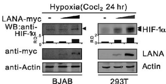
FIG. 2. The KSHV-encoded nuclear protein LANA regulates HIF-1 \alpha expression in a dose-dependent manner. Ten million hypoxia-treated Burkitt lymphoma BJAB cells and HEK 293T cells were transfected with different doses of plasmid pA3M/LANA normalized by the pA3M vector and maintained under hypoxic conditions. After 24 h of transfection, the cells were harvested and lysed for Western blot (WB) analysis using antibodies against HIF-1 \alpha , myc, or \beta -actin. The data show that HIF-1 \alpha expression was increased by LANA in a dose-dependent manner. RD, relative density.
