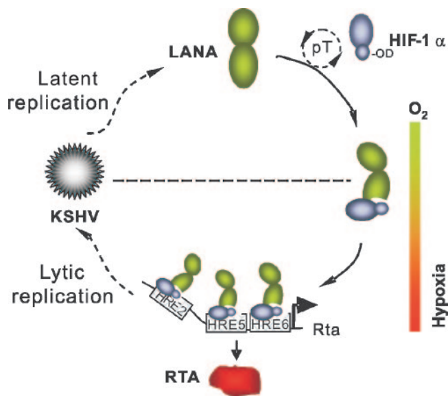
FIG. 9. Hypothetical model for KSHV-encoded latent protein LANA interaction with HIF-1 \alpha during hypoxia and KSHV reactivation. During KSHV latent replication, the essential latent protein LANA induces the transcription of the HIF-1 \alpha promoter (pT) during hypoxia. The expressed HIF-1 \alpha interacted with LANA to activate the transcription of the Rta promoter, which contains hypoxia response elements (HRE-2, HRE-5, and HRE-6). The highly expressed RTA protein drives virus to lytic replication. OD, oxygen-dependent domain.
