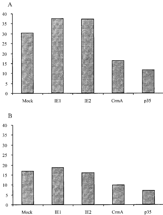
FIG. 2. CrmA and p35 reduce Vpr-induced apoptosis. Transfection efficiencies were analyzed by flow cytometry at 48 h posttransfection. The data shown is representative of three independent experiments. (A) Bar graph representing Annexin V staining of cells transfected with the indicated viral anti-apoptosis gene and infected with HIV-1 NL4-3 Thyenv(-)/VSV-G. The percentage of Annexin V staining is represented on the y axis. The data indicated are results from 72 h posttransfection and 48 h postinfection. (B) Bar graph representing Annexin V staining of cells transfected with the indicated viral anti-apoptosis gene and infected with HIV-1 NL4-3 Thyenv(-)VprX/VSV-G. The percentage of Annexin V staining is represented on the y axis. The data indicated are results from 72 h posttransfection and 48 h postinfection.
