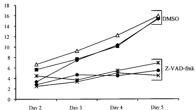
FIG. 4. Synthetic caspase inhibitor protects human T cells from Vpr-induced apoptosis. SupT1 cells ( 4 \times 10^5 ) were mock infected or infected with HR'Vpr for 4 h in the presence of 10 \mu g of polybrene per ml. Following infection, cells were washed and DMSO or 100 \mu M z-VAD-fmk, dissolved in DMSO, was added. Fresh DMSO or z-VAD-fmk was added every 24 h for the duration of the experiment. The experiment was carried out in triplicate, and percentage of apoptosis is plotted against time for HR'Vpr-infected cells treated with either DMSO or z-VAD-fmk as indicated. The difference between estimated mean response at day 3 is significantly lower for z-VAD treatment than for treatment with DMSO ( P < 0.005 by testing contrasts for fixed effects in a mixed linear model for repeated measurements) (30).
