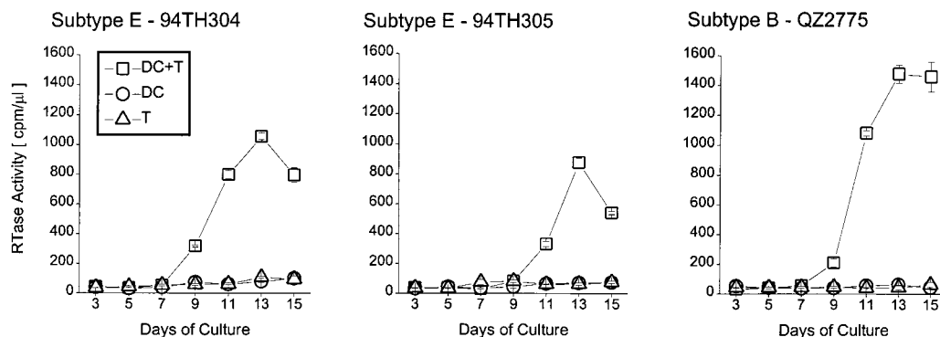
FIG. 2. Purified cutaneous DCs do not support the growth of HIV-1 of subtype B or E. Aliquots of 10^5 sorted DCs (DC), 10^5 sorted T cells (T), and mixtures of the two (DC+T; 1:2) were exposed to 100 TCID 50 of the indicated HIV-1 isolate and cultured for 15 days. Productive infection was assessed by monitoring the culture supernatants for the presence of reverse transcriptase (RTase) activity (mean counts per minute \pm standard errors of the means of triplicate samples are shown). The results from one of four similar experiments are depicted.
