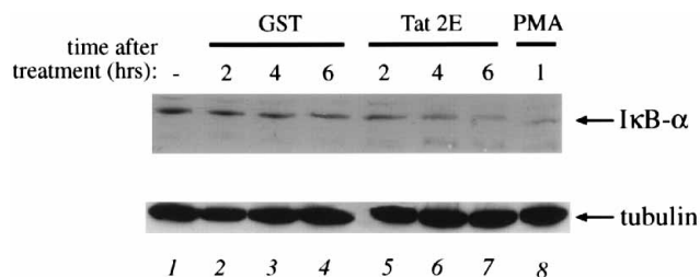
FIG. 6. Immunoblotting analysis of I \kappa B- \alpha in HL3T1 cells. Cell extracts were prepared at different times after lipofection with GST (lanes 2 to 4) or Tat 2E (lanes 5 to 7) or after treatment with PMA (lane 8), as indicated. I \kappa B- \alpha and tubulin (as a control for monitoring protein loading in each lane and transfer efficiency) were detected by Western blotting (immunoblotting) with specific antibodies. Tat and PMA treatments induce degradation of I \kappa B- \alpha .
