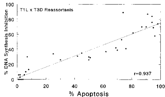
FIG. 4. Correlation between the capacities of T1L × T3D reassortant viruses to inhibit cellular DNA synthesis and to induce apoptosis. Each point represents a single reassortant virus. Data are derived from Table 2 and reference 55.
