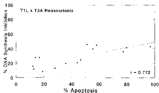
FIG. 3. Correlation between the capacities of T1L × T3A reassortant viruses to inhibit cellular DNA synthesis and to induce apoptosis. Each point represents a single reassortant virus. Data are derived from Table 1.
