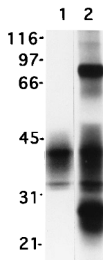
FIG. 5. SDS-PAGE analysis of proteins immunoprecipitated by anti-peptide antibody anti-BZLF2 (lane 1) or monoclonal antibody F-2-1 (lane 2) from induced Akata cells labeled with [ ^3 H]glucosamine for 20 h at 6 h postinduction. Sizes are indicated in kilodaltons.
