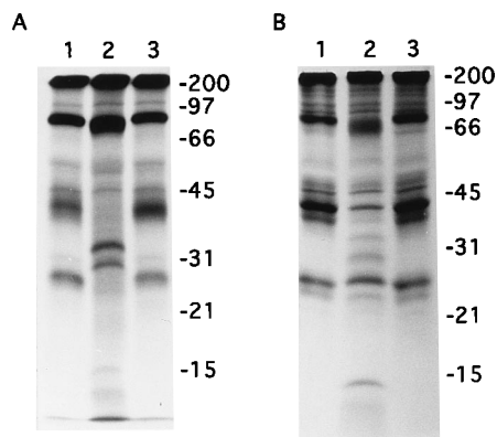
FIG. 4. SDS-PAGE analysis of proteins immunoprecipitated by antipeptide antibody anti-gL from Akata virus labeled with ^{125}\text{I} (A) or with induced Akata cells labeled with ^{35}\text{S} cysteine (B) for 20 h at 6 h postinduction. Before electrophoresis, proteins were incubated overnight in digestion buffer alone (lanes 1), with endoglycosidase F (lanes 2), or with neuraminidase and O -glycanase (lanes 3). Sizes are indicated in kilodaltons.
