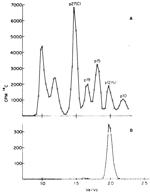
FIG. 2. Comparison of proteins from MC29 virus with protein from viral RNP's by gel filtration in 6 M GuHCl. A mixture of 14 C-labeled amino acids was used to label virus in vivo . RNP's were isolated as in Fig. 1A, dialyzed rapidly to get rid of sucrose, lyophilized, and subjected to gel filtration in 6 M GuHCl and 0.01 M DTT. The protein pattern for whole virus is shown in panel A, and the pattern for RNP's in panel B. For protein designations see legend to Table 1.
